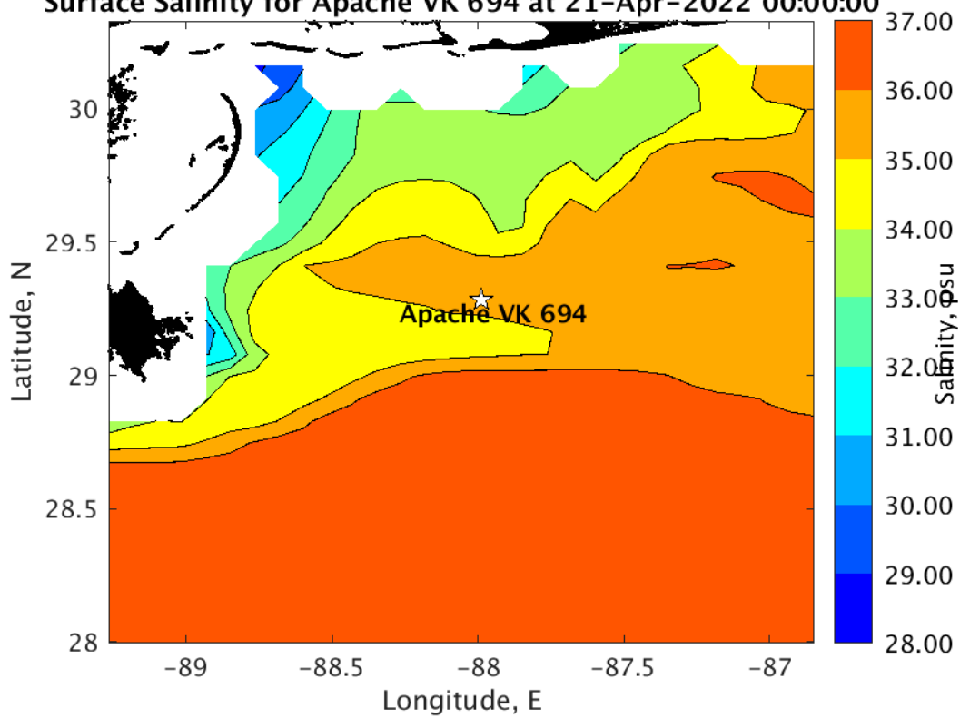
Surface Salinity for Apache VK 694 at 21-Apr-2022 00:00:00
